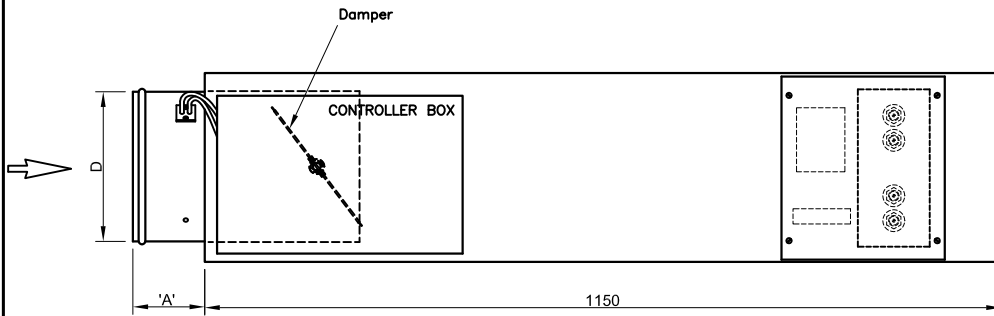
FRONT VIEW
