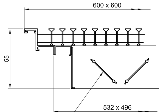
Opposed blade damper
