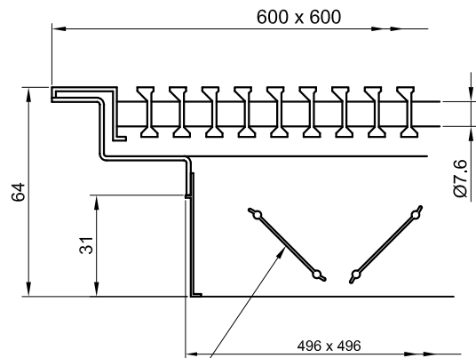
Opposed blade damper
