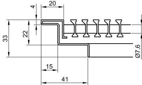
Typical Corner Detail
