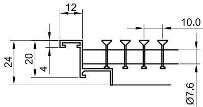
Typical Corner Detail
