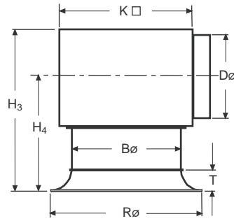
Model HCSD- H...
